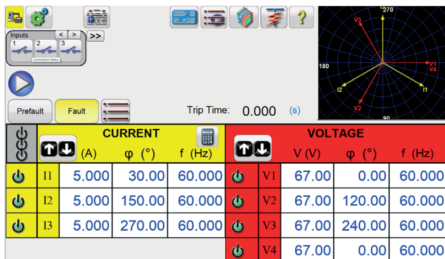
Figure 2: RTMS advanced user interface
