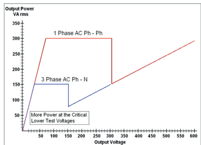
Figure 5: Voltage output power curve
