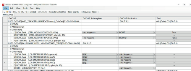
Figure 6: Megger GOOSE Configurator software
