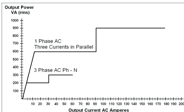
Figure 4: Current output power curve
