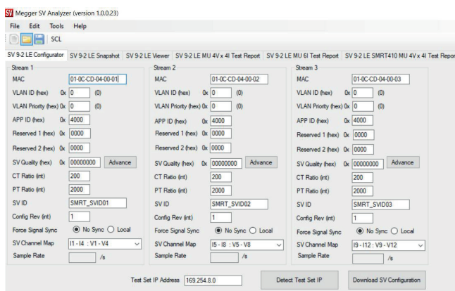
Figure 7: Megger Sampled Values Configurator
