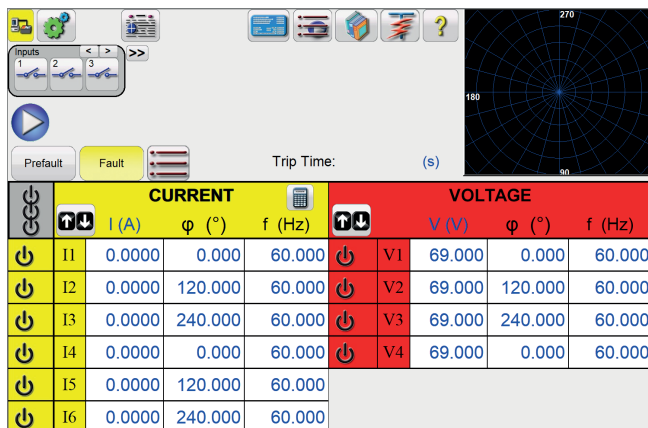
Figure 2: RTMS advanced user interface
